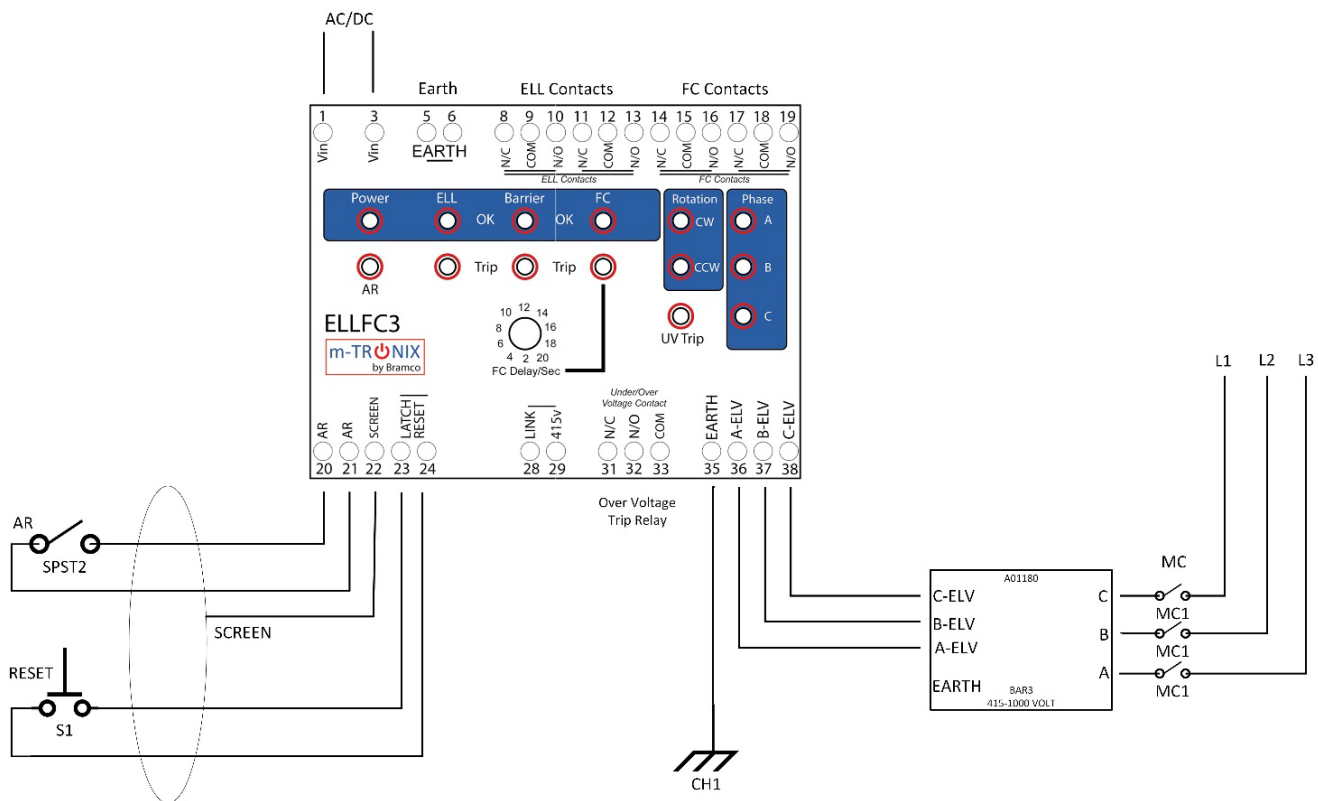
ELLFC3 Wiring Diagram
